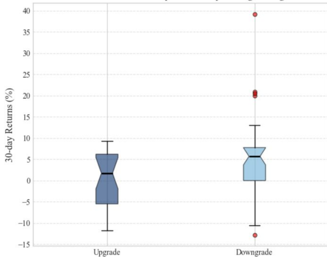
Distribution of 30-day Returns by Rating Change
